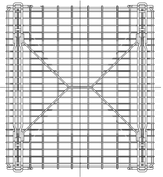
Drawing of Steel Wiremesh Containers with Upper and Lower Doors for Pallet Truck Loading and Unloading
